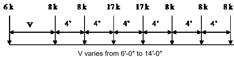
Figure 13.1-6 Notional Rating Load (NRL) (LRFR & LFR Methods)
