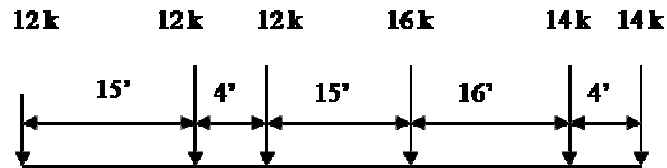
Figure 13.1-5 Type 3-3 (LRFR & LFR Methods)
