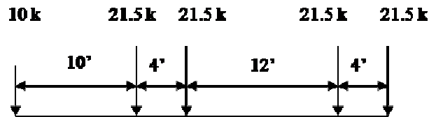
Figure 13.1-8 Overload 1* (LRFR & LFR Methods)
