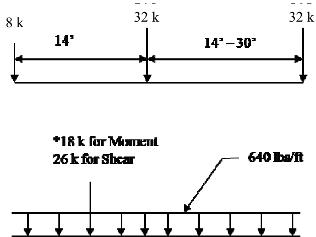
Figure 13.1-2 HS-20 Load (LFR Method)
