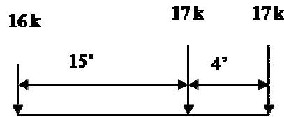
Figure 13.1-3 Type 3 (LRFR & LFR Methods)
