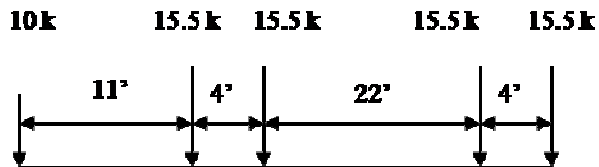
Figure 13.1-4 Type 3S2 (LRFR & LFR Methods)
