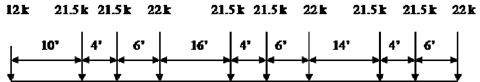
Figure 13.1-9 Overload 2* (LRFR & LFR Methods)
