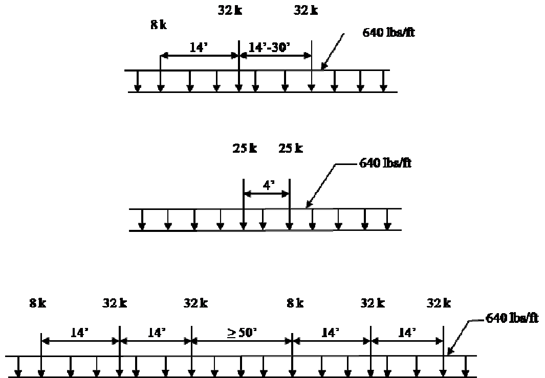
Figure 13.1-1 HL-93 Load (LRFR Method)
