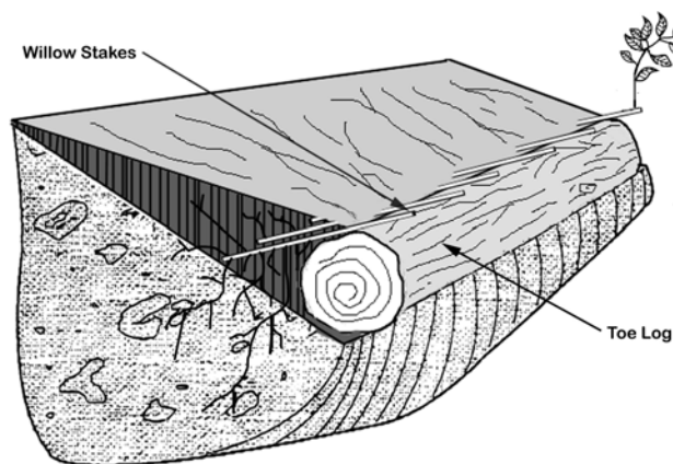
Figure 740.8 Toe Log Technique
