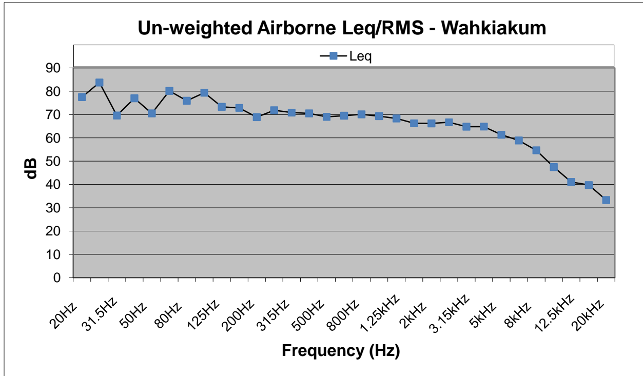
Figure 5: Comparison of Wahkiakum un-weighted airborne frequency distributions for the Leq/RMS metric using a vibratory hammer.
