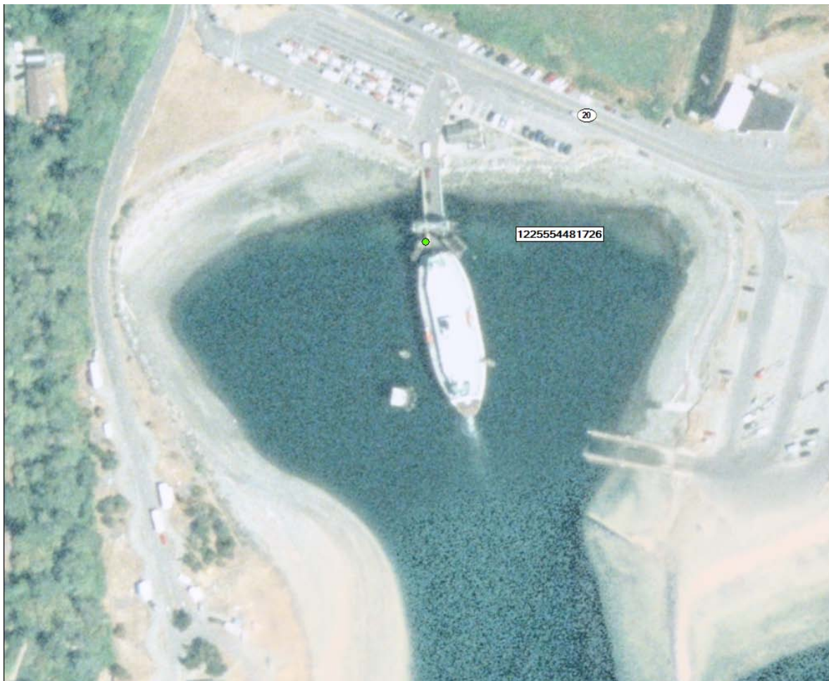
Figure 7: Location of airborne noise monitoring at the Keystone Ferry Terminal.
