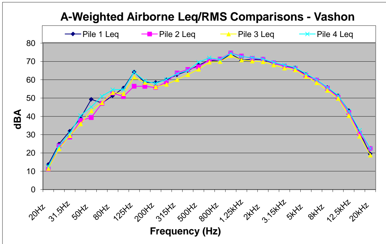
Figure 2: Comparison of Vashon A-weighted airborne frequency distribution for the Leq/RMS metric using a vibratory hammer.
