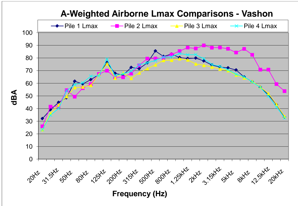
Figure 3: Comparison of Vashon A-weighted airborne frequency distributions for the Lmax metric using a vibratory hammer.
