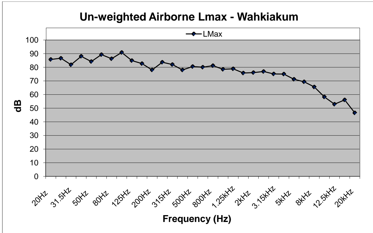
Figure 6: Comparison of Wahkiakum un-weighted airborne frequency distributions for the Lmax metric using a vibratory hammer.
