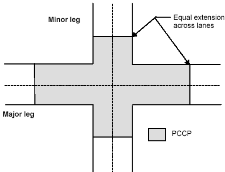
Figure 8.1. PCCP Intersection Limits
