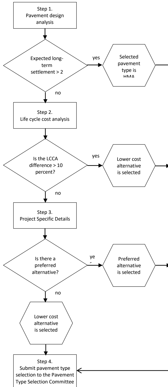
Figure 4.1. Pavement Type Selection Flow Chart
